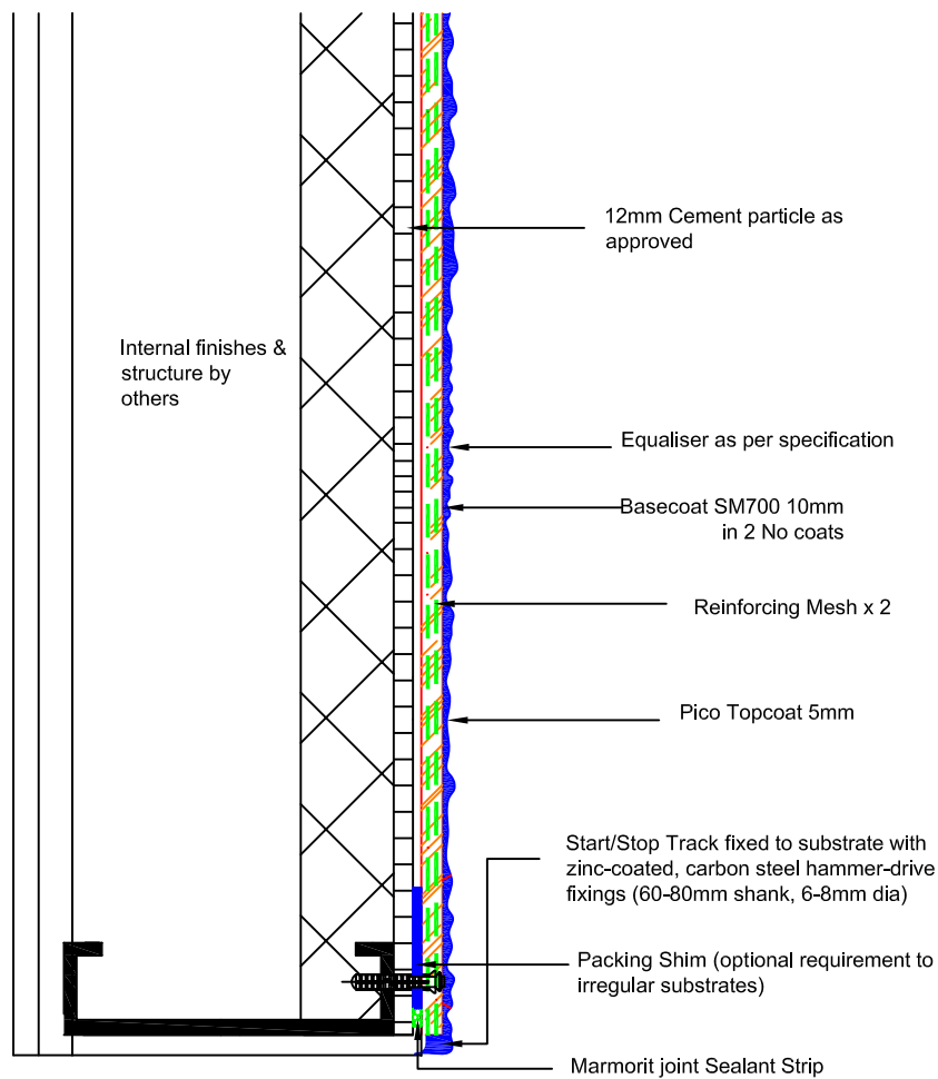
TYPICAL SECTION Scale: 1 : 2
