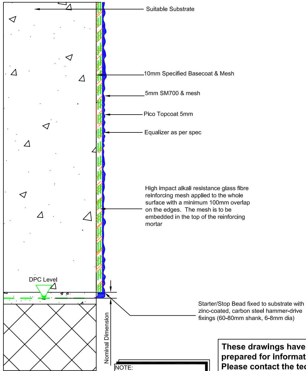
TYPICAL SECTION Scale: 1 : 2
