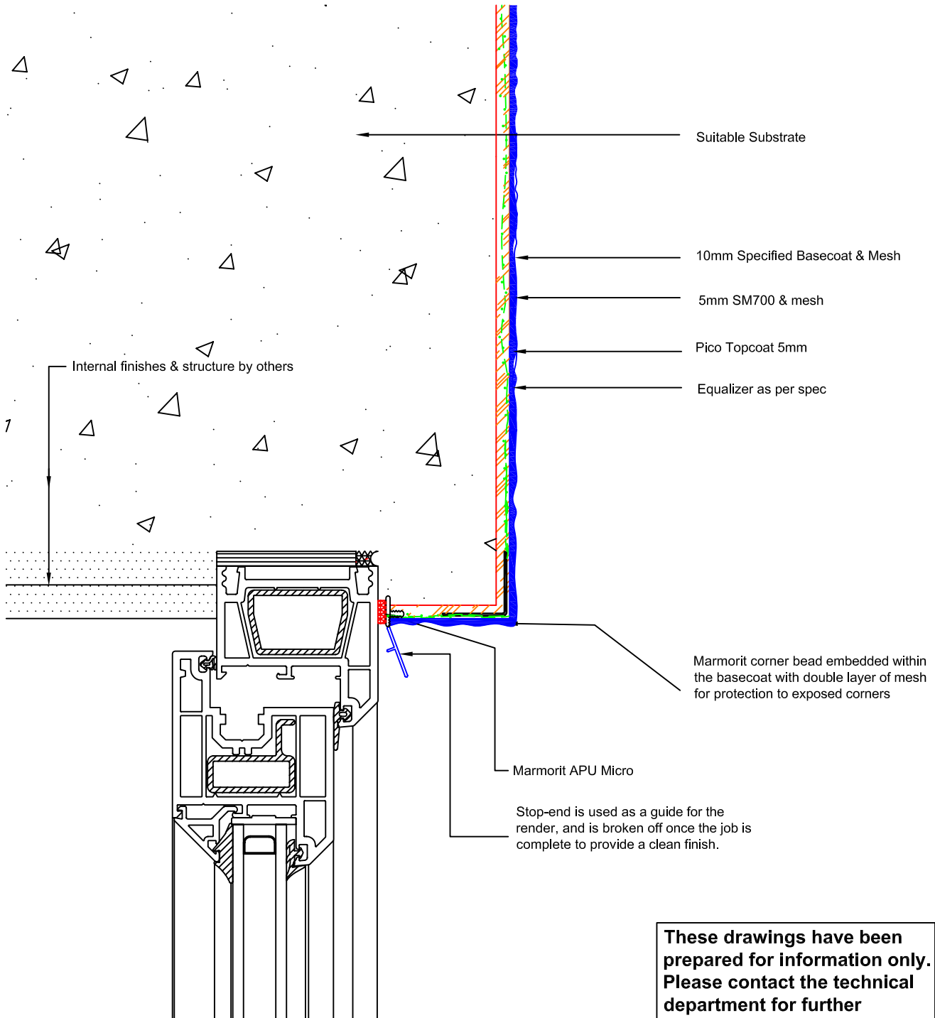
WINDOW HEAD SECTION Scale: 1 : 2
