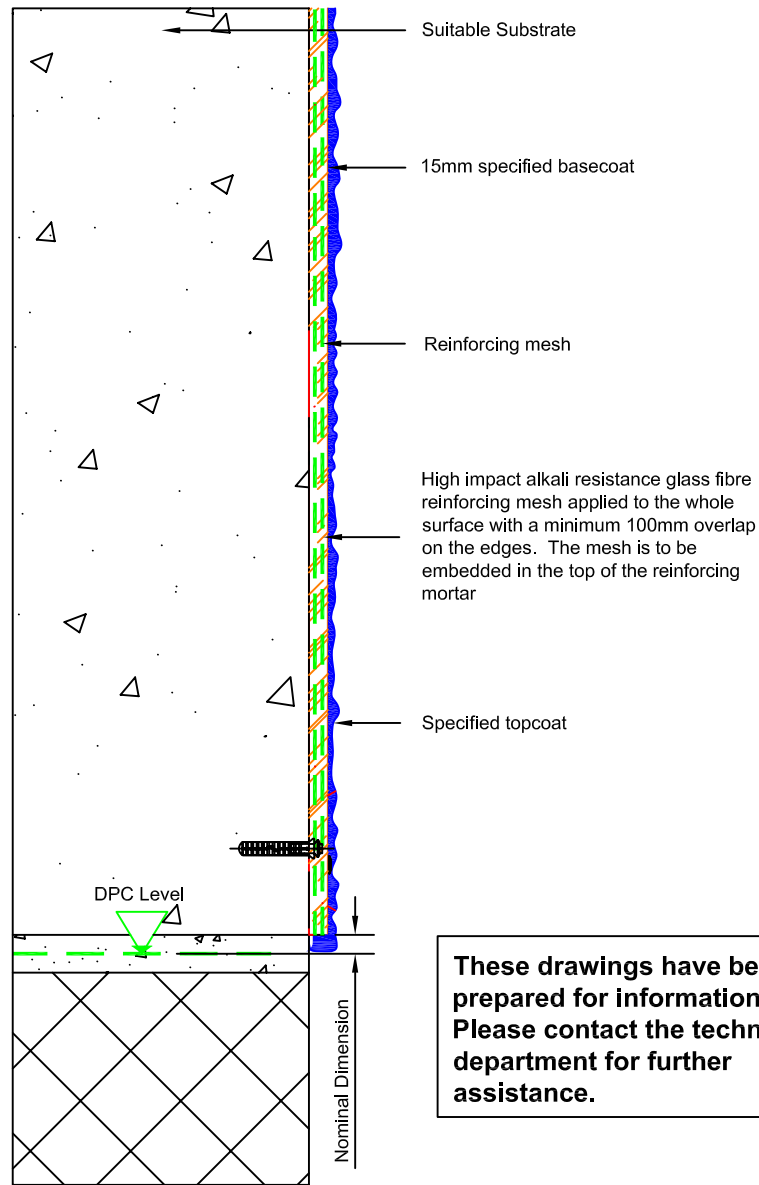
TYPICAL SECTION Scale: 1 : 2
