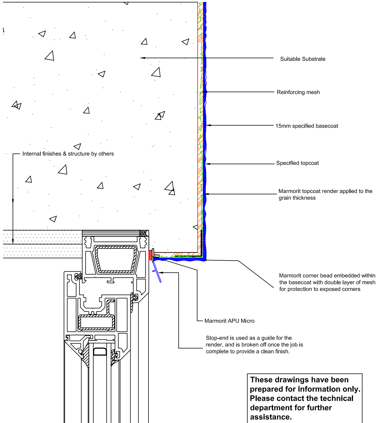
WINDOW HEAD SECTION Scale: 1 : 2
